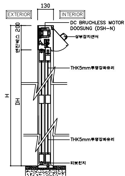
VERTICAL SECTION (OPEN)
