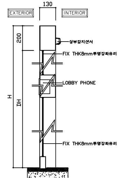
VERTICAL SECTION (FIX)
