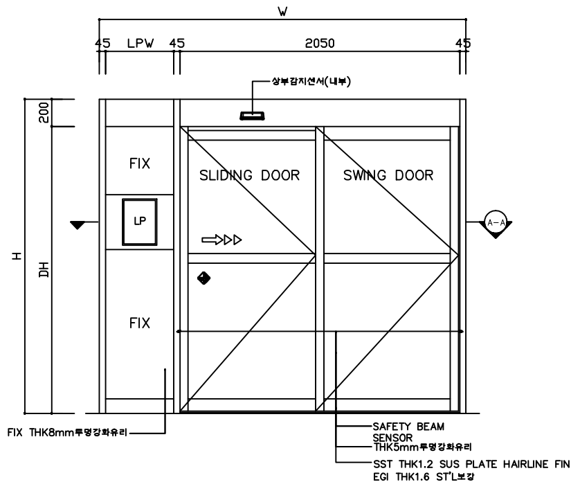
ELEVATION [EXTERIOR]
